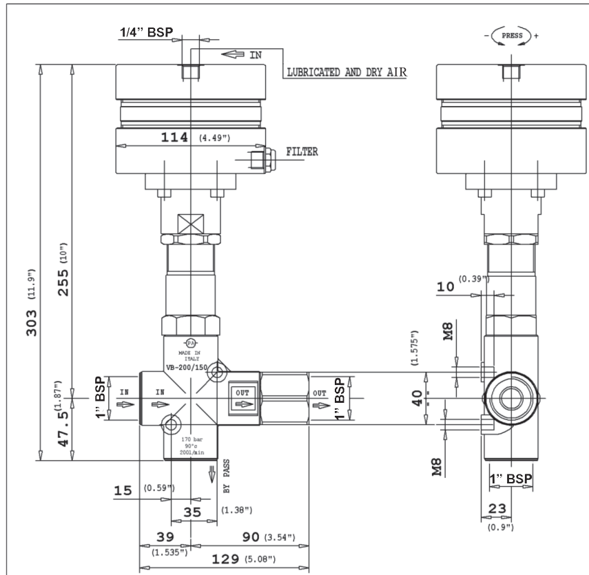
Dimensional Drawing - mm (Inches)
