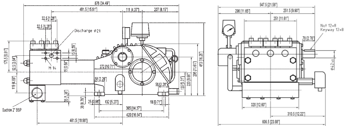
Compact Head M
