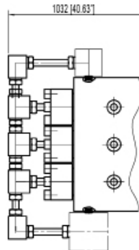
High Pressure Head A 29,000 PSI (2000 Bar)
