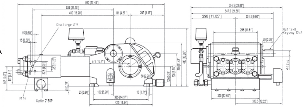
High Pressure Head A
