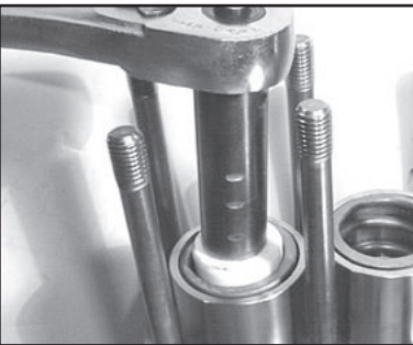
10. Tighten the tension screws (29C) to 26.5 ft.-lbs. (35 Nm). The plunger pipe (29B) should not be strained by over tightening of the tension screw (29C) or through damage to the front surface of the plunger; otherwise, it will probably break.
