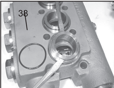
7. Remove seal case (37) from valve casing (43) and inspect o-ring (38).
