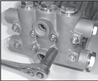
4. Loosen the 8 nuts (49A) with a 19mm wrench. Tap the back of the manifold (43) with a rubber mallet to dislodge and slide off the studs (49).
