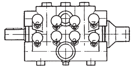
11. Place valve casing (43) over studs and push firmly until seated against the crankcase (1). Tighten the hexagon nuts (49A) in a crosswise pattern (shown above) to 59 ft.-lbs. (80 Nm).
