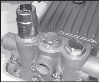
1. With a 30mm wrench, remove the (3) plugs (48).
