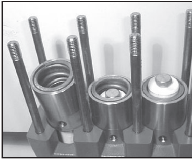
5. Pull seal sleeves (35) out of guides in crankcase (1).
