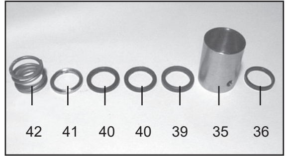
6. Remove the tension spring (42), support ring (41), v-sleeves (40), pressure ring (39), from the seal sleeve (35). Examine seals (36) carefully and replace if worn. Clean all parts.
