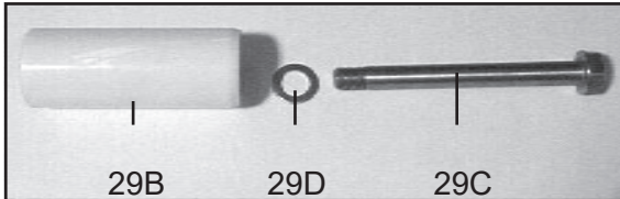
8. Check plunger surface (29B). If plunger pipe is worn, loosen tension screws (29C) and pull off plunger pipe to the front. Clean front surface of plunger (25) thoroughly. Apply a thin coat of Loctite to the tension screw threads (29C). Note: Care must be taken that no glue gets between the plunger pipe (29B) and the centering sleeve (29A). Add new copper ring (29D).
