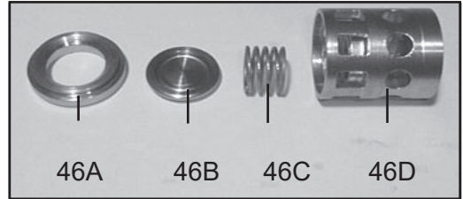
3. Loosen valve seats (46A) from spacer pipe (46D) by lightly hitting the valve plate (46B) with a plastic stick. Check sealing surface and replace worn parts. Reassemble with new o-rings (44A) and oil them before installing. Tighten up tension plugs (48) to 107 ft.-lbs. (145 Nm).
