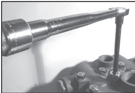
11. Place valve casing (43) over studs and push firmly until seated against the crankcase (1). Tighten the hexagon nuts (49A) in a crosswise pattern (shown above) to 59 ft.-lbs. (80 Nm).
