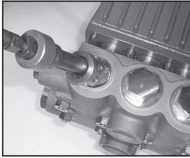
2. Remove the complete valve assembly (46) with valve pullers.
